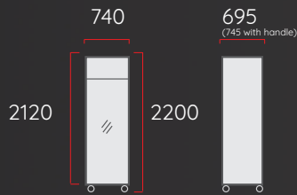
1 Door Top Mount Fridge
