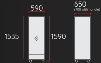
1 Door Bottom Mount Fridge, Lit Sign
