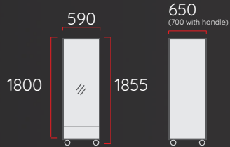
1 Door Bottom Mount Fridge
