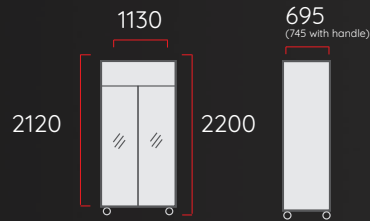
2 Door Top Mount Fridge
