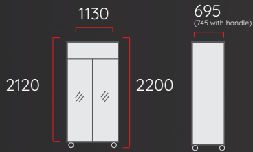
2 Door Top Mount Customisable Fridge
