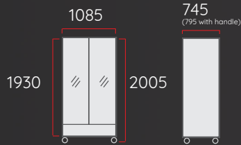
2 Door Bottom Mount Customisable Fridge
