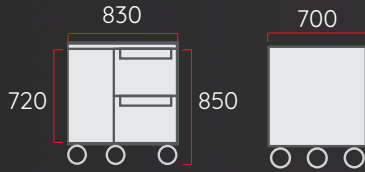
1 Bay, 2 Drawer, Underbench Fridge
