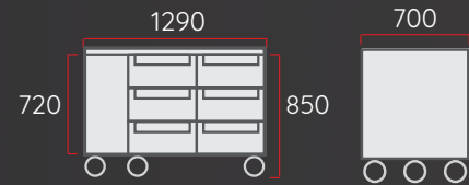
2 Bay, 3 Drawer, Underbench Fridge
