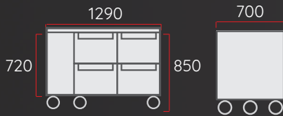
2 Bay, 2 Drawer, Underbench Fridge
