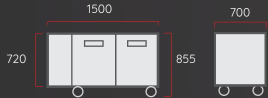
3 Bay, 3 Door Underbench Freezer
