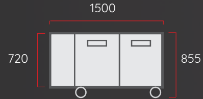
2 Bay, 2 Door Underbench Large Fridge
