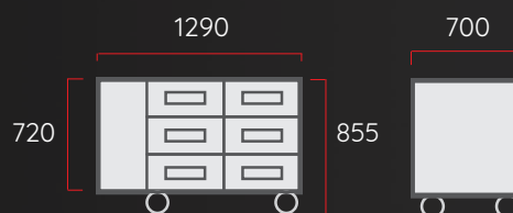
2 Bay, 6 Drawer Underbench Fridge
